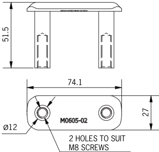
Bolt-Through Strap
