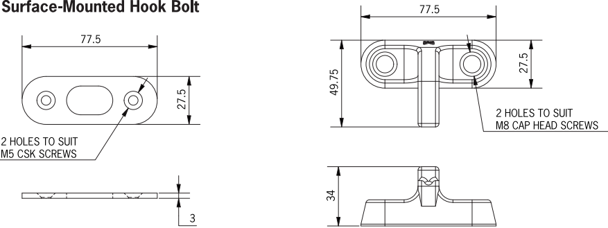
Surface-Mounted Hook Bolt
