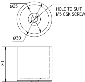
Mortice-Fitted Hinge Bolt
