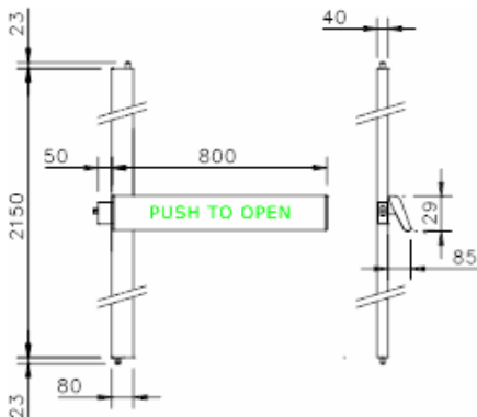
Drawing Not to Scale. Drawing shows outward opening unit.
